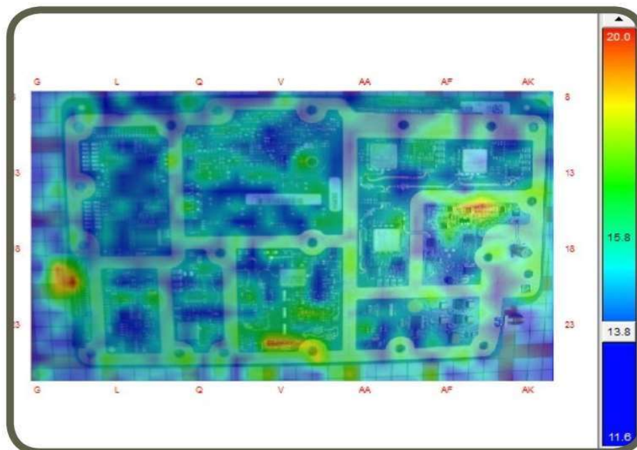
Spatial Scan of the Bad Board at the IF frequency
