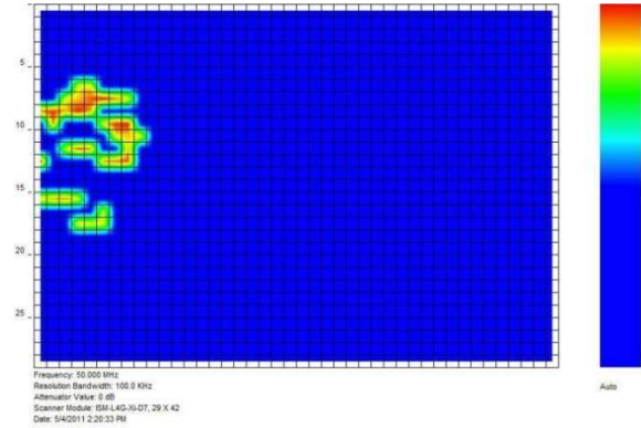
EMScanner spatial scan at 50MHz with no noise injection.
