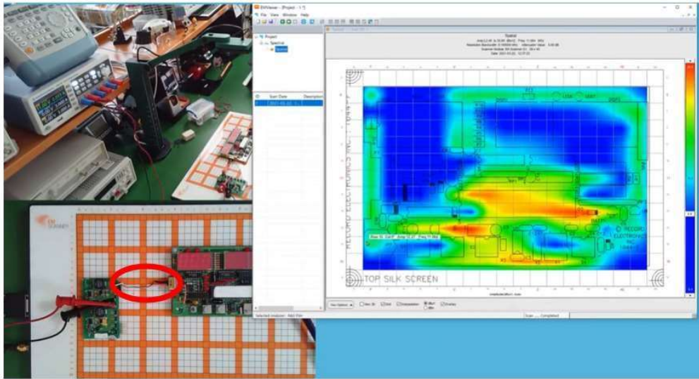
Unfiltered connection to power supply circled in red
