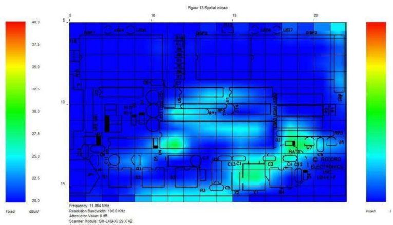
Taximeter PCB test with Noise by at least 8dBuV.
