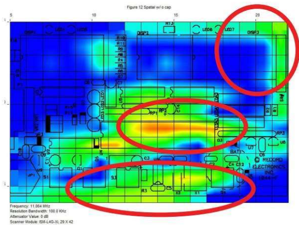
Taximeter PCB test with no capacitor – noise capacitor reduces circled in red.
