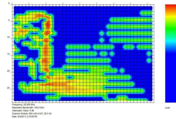
EMScanner spatial scan at 50MHz with noise injection at right edge of board.
